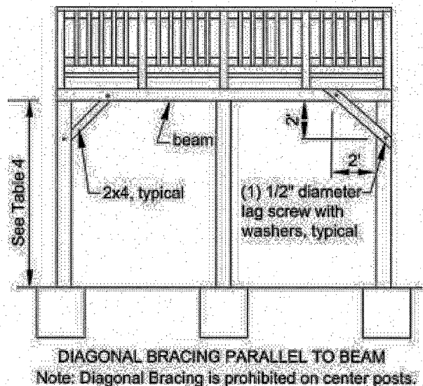
Figure 10. Diagonal Bracing.
