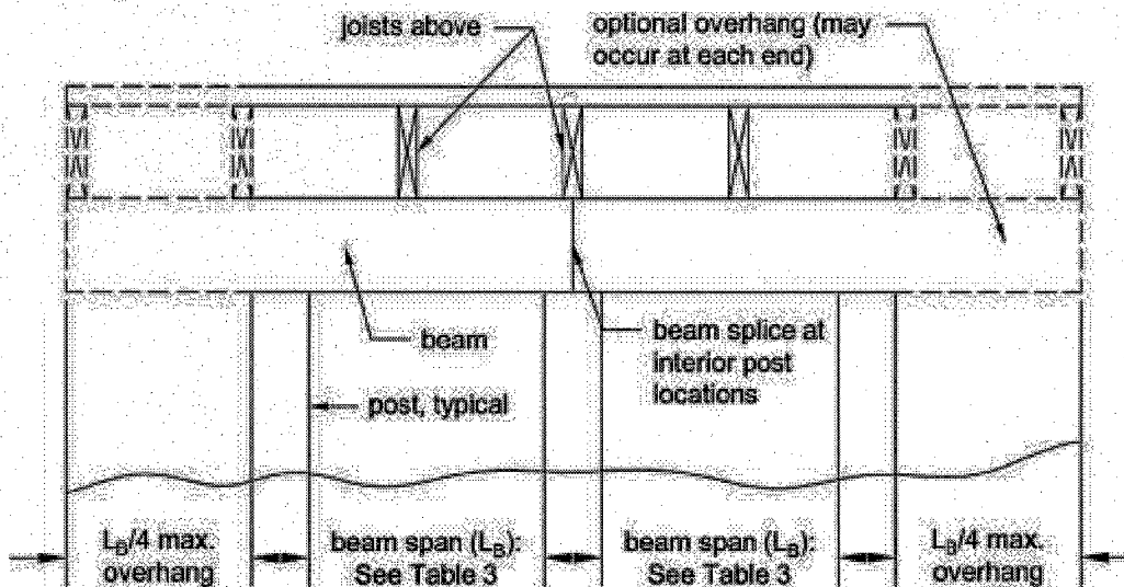
Figure 3. Beam Span.
